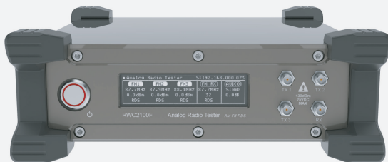
RWC2100F Front View 2.81" OLED Display Power On/Off Switch 3 x TX, 1 x RX Port
