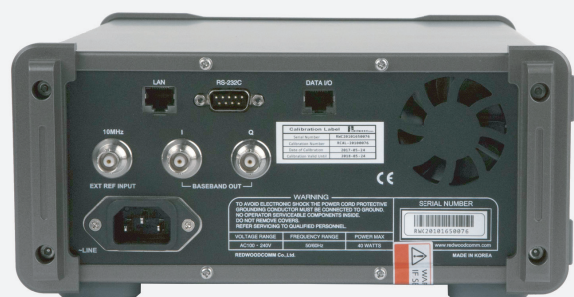
RWC2010B Rear View LAN, RS-232, DATA I/O 10 MHz Reference In I/Q Baseband Out AC Power Input
